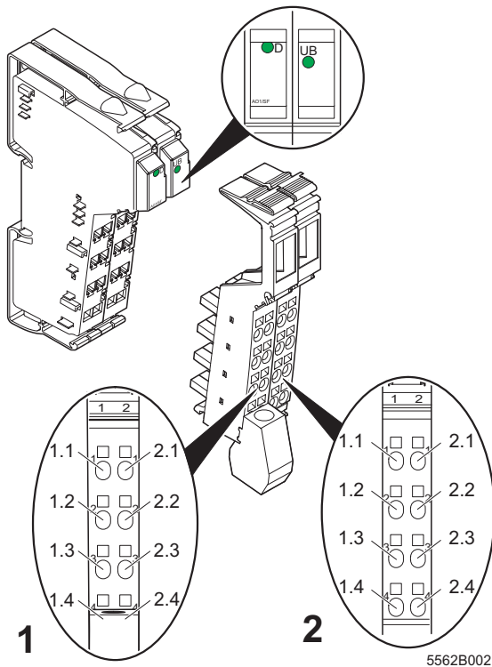
Figure 2 IB IL AO 1/SF with appropriate connectors
