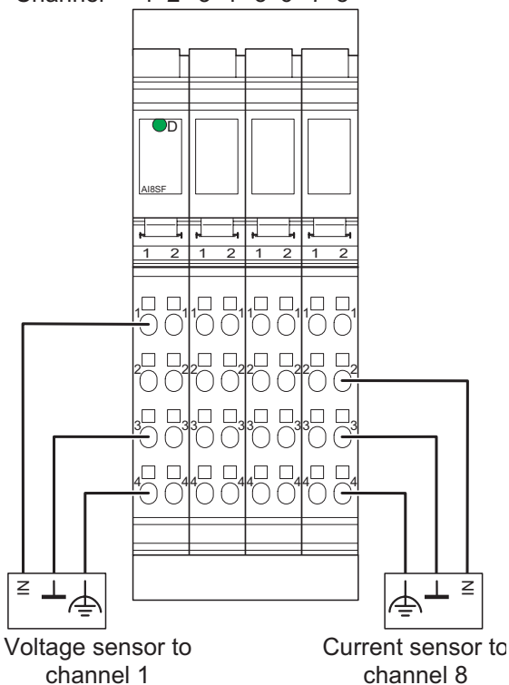
Figure 5 Connection of active sensors using 2-wire technology with shield connection
