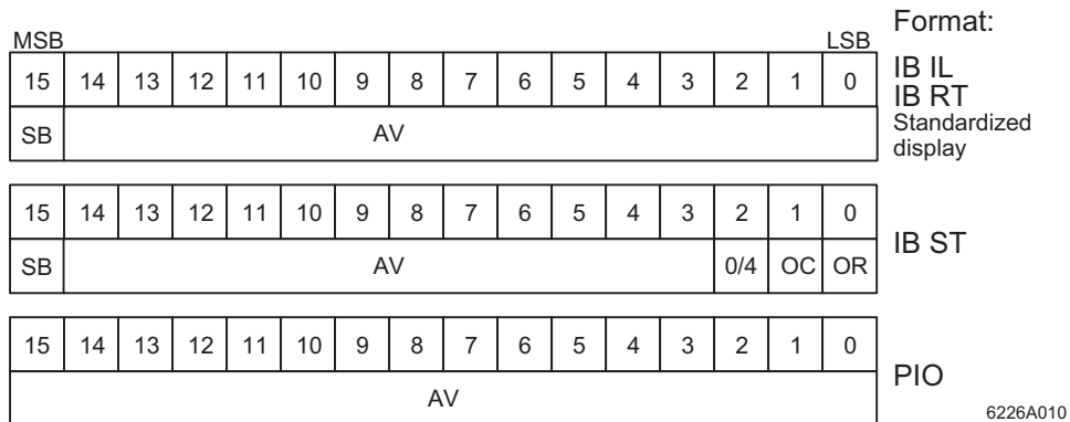
Figure 8 Representation of the measured values in the different formats
