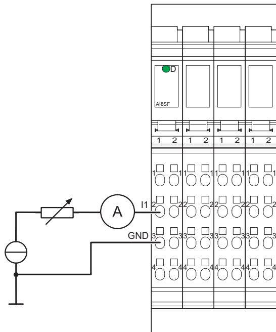
Figure 13 Measuring currents
