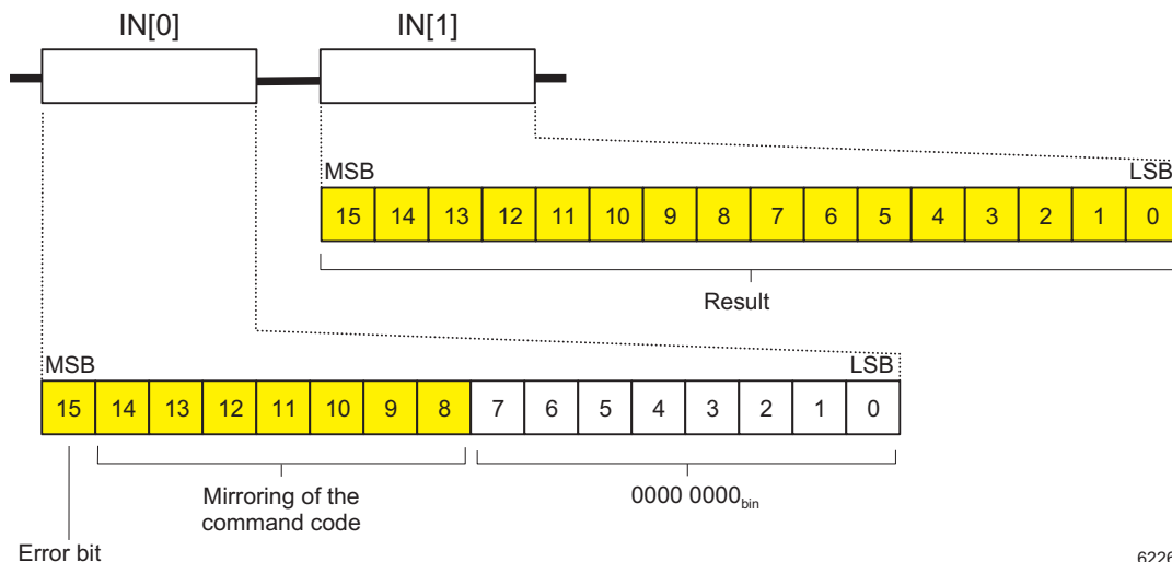
Figure 7 Process data input words
