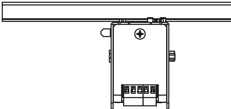
Fig. 4: Top View - JX2-OD8
