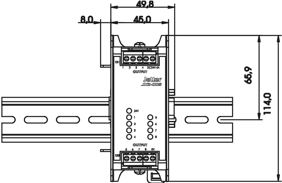
Fig. 2: Front View - JX2-OD8
